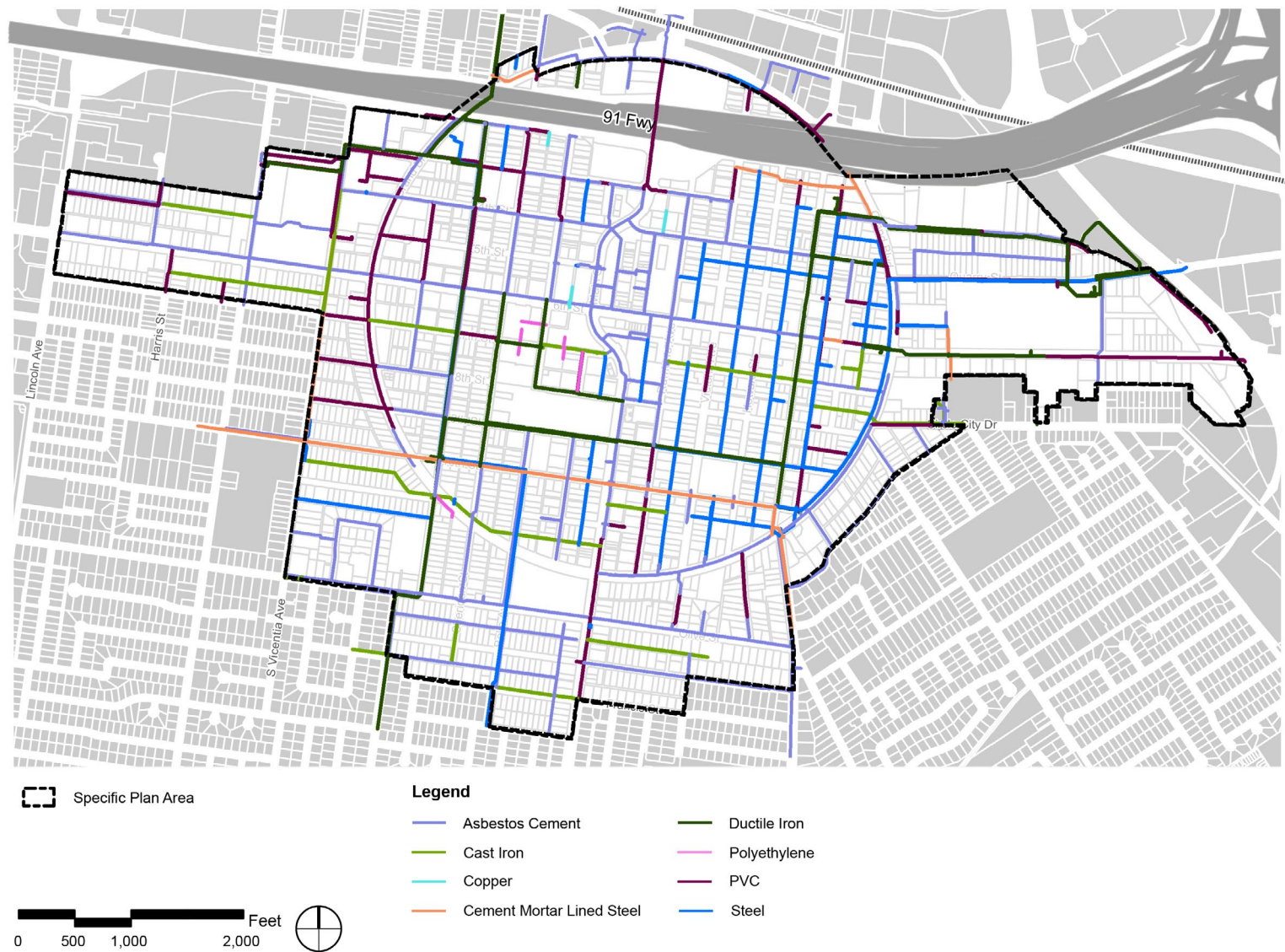
Figure 6-2: Existing Water System - Pipe Materials
