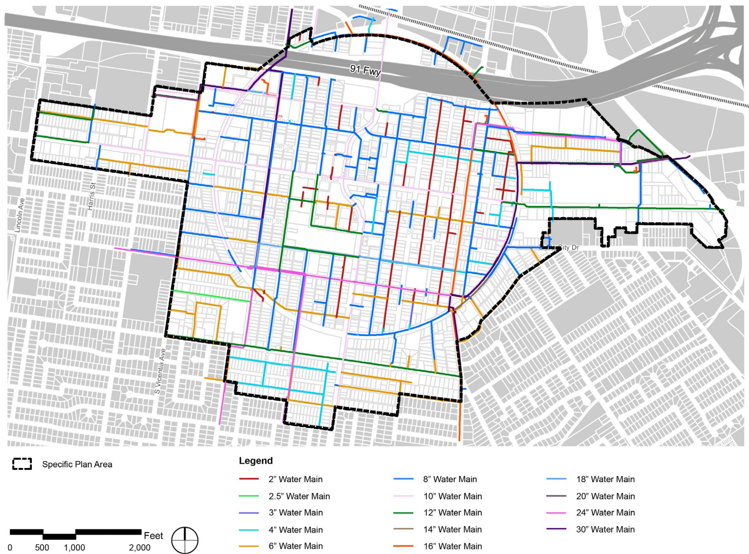
Figure 6-1: Existing Water System - Pipe Size
